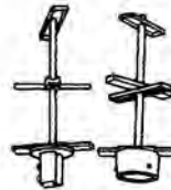
Style 556 Cap for 2" Std. Pipe Cap for 2 1/2" Std. Pipe Separators Center Rod Dome Nut Four Way Complete Two Way Complete Specify Center Hole Taped or Untaped
