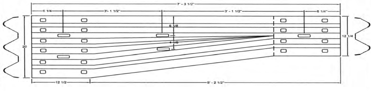
THRIE BEAM TRANSITION SECTION
