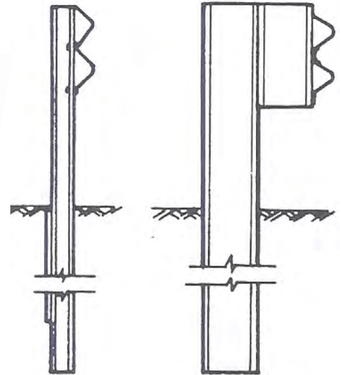
STEEL POSTS and BLOCKS
